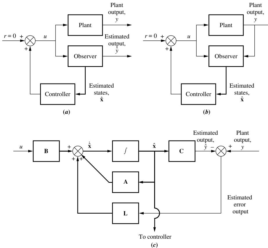
FIGURE 12.11 State-feedback design using an observer to estimate unavailable state variables: a. open-loop observer; b. closed-loop observer; c. exploded view of a closed-loop observer, showing feed-back arrangement to reduce state-variable estimation error
