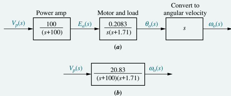
FIGURE 4.32 Antenna azimuth position control system for angular velocity: a. forward path; b. equivalent forward path
