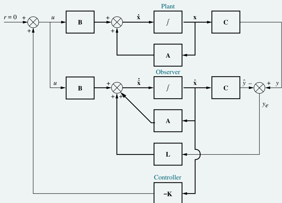
FIGURE 12.23 Conceptual state-space design configuration, showing plant, observer, and controller
