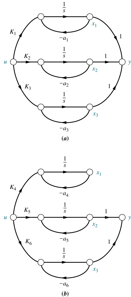
FIGURE 12.15 Comparison of a. observable, and b. unobservable systems
