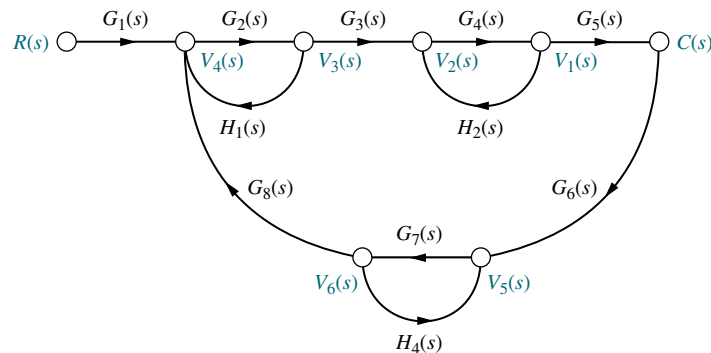
FIGURE 5.21 Signal-flow graph for Example 5.7
