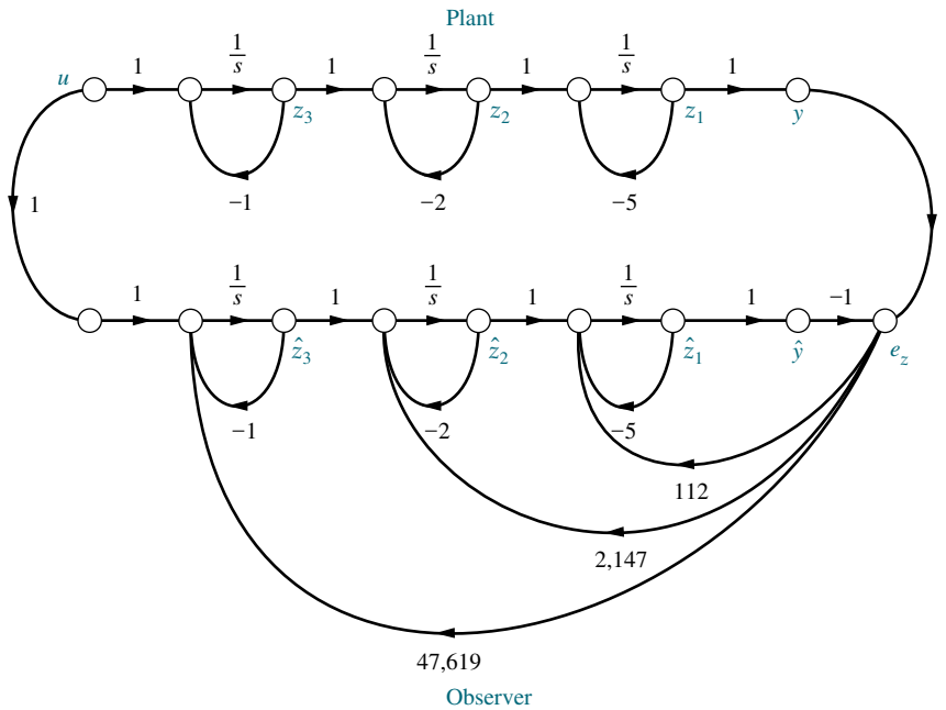
FIGURE 12.18 Observer design
