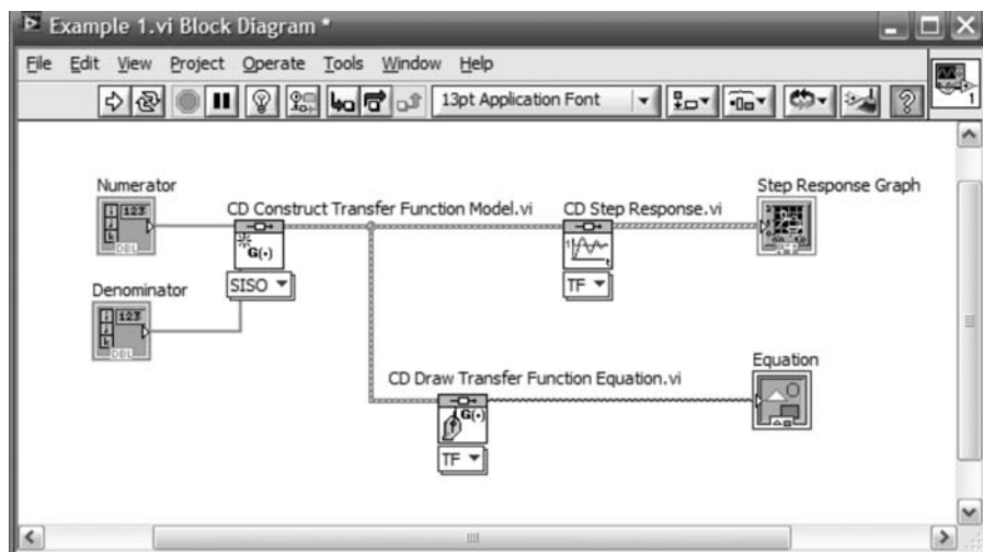
FIGURE D.7 Block Diagram window: a. with Control Design blocks and interfaces; (figure continues)
