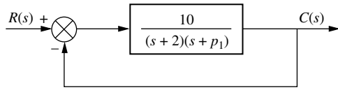
FIGURE 8.24 System requiring a root locus calibrated with p_1 as a parameter
