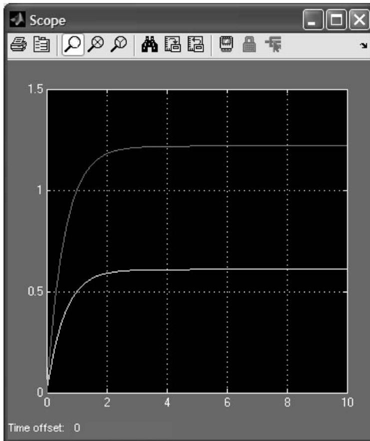
FIGURE C.12 Scope window after simulation of Example C.2 stops. The lower curve is the output with saturation
