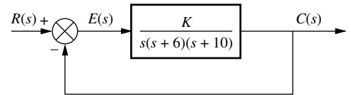
FIGURE 9.37 Uncompensated system for Example 9.6
