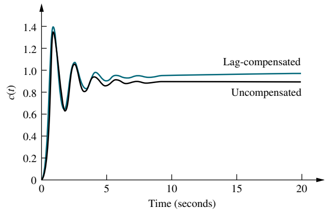
FIGURE 9.13 Step responses of uncompensated and lag-compensated systems for Example 9.2
