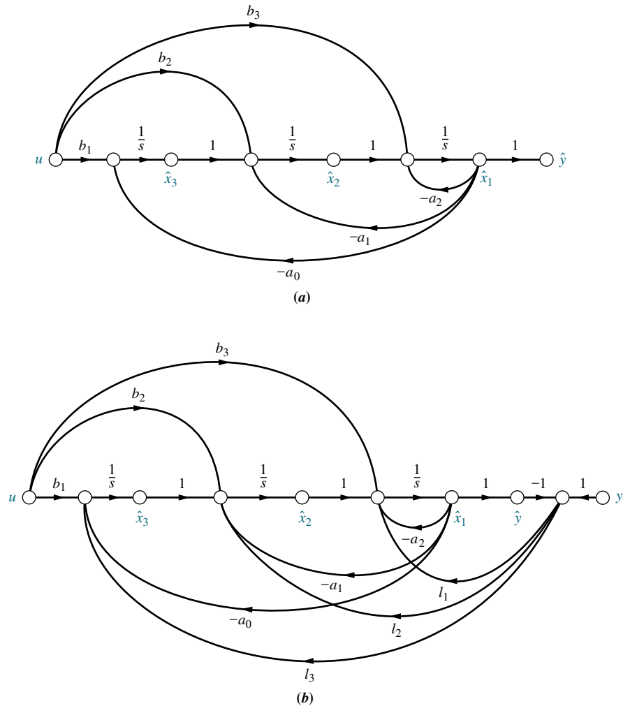
FIGURE 12.12 Third-order observer in observer canonical form: a. before the addition of feedback; b. after the addition of feedback
