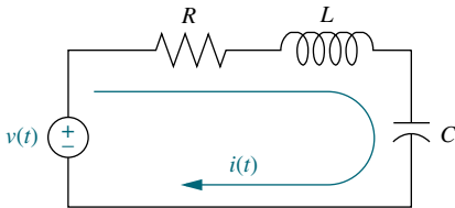
FIGURE 3.2 RLC network
