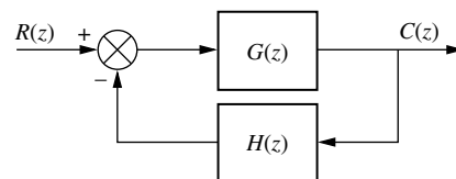
FIGURE 13.20 Generic digital feedback control system
