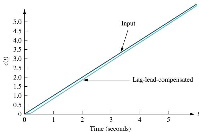
FIGURE 9.43 Improvement in ramp response error for the system of Example 9.6: a. lead-compensated; b. lag-lead-compensated
